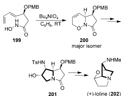
Scheme 37. Total synthesis of (+)-loline. PMB = para -methoxybenzyl.
