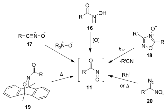
Scheme 2. Common synthetic routes to nitrosocarbonyl species.
