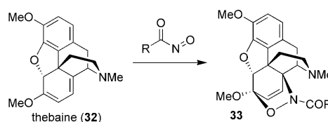
Scheme 5. The cycloaddition reported by Kirby and Sweeny. [31]
