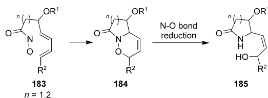
Scheme 34. General route to monocyclic alkaloids.
