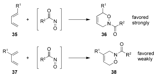
Scheme 6. General selectivity observed for unsymmetrical dienes.
