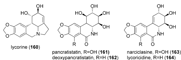
Figure 11. Structures of amaryllidacea alkaloids.
