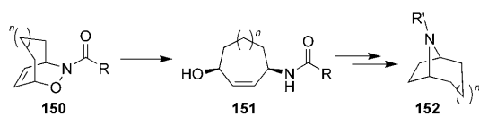
Scheme 28. General synthetic route to tropane alkaloids.
