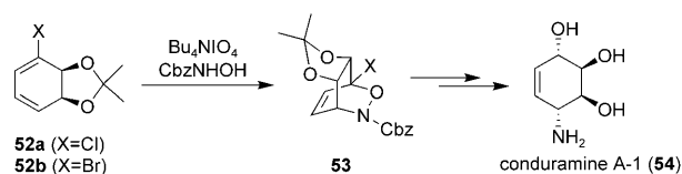
Scheme 8. Stereoselective nitrosocarbonyl HDA reaction in the presence of a chiral diene. Cbz = benzyloxycarbonyl.
