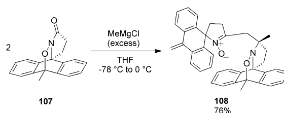
Scheme 20. An unusual reaction with a Grignard reagent.
