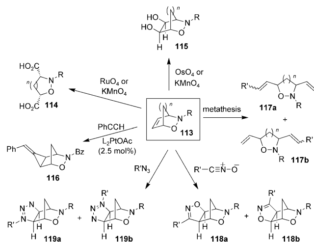
Scheme 22. Examples of alkene modification of bicyclic cycloadducts. Bz = benzoyl.
