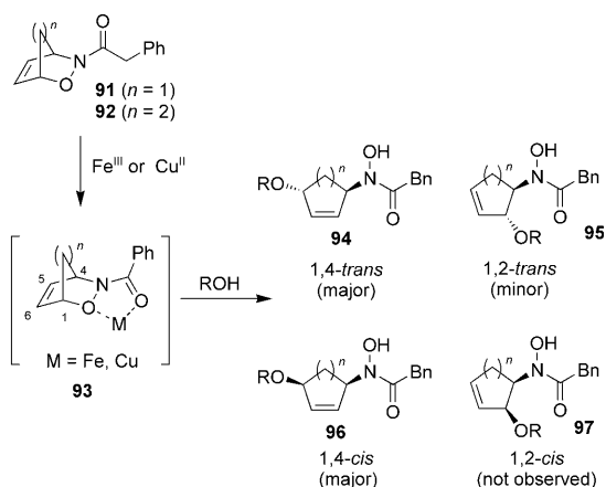
Scheme 17. Lewis acid mediated cleavage of a C–O bond. Bn = benzyl.
