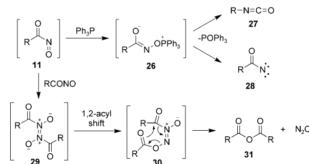
Scheme 4. Other reactions of nitrosocarbonyl compounds.
