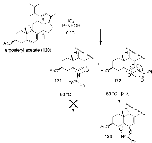
Scheme 23. [3,3] Rearrangement of an ergosteryl cycloadduct.
