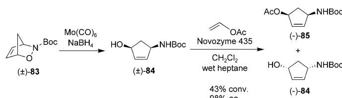
Scheme 15. Enzymatic resolution of a racemic alcohol.
