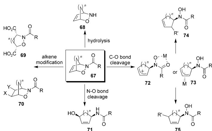
Scheme 12. Modification of bicyclic 3,6-dihydro-1,2-oxazines.
