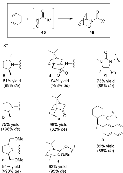
Figure 6. Examples of chiral nitrosocarbonyl compounds.
