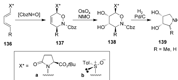
Scheme 26. Synthetic route to pyrrolidines. NMO = 4-methylmorpholine N -oxide, Tol = tolyl.
