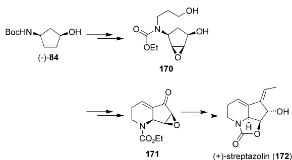
Scheme 31. Synthetic route to (+)-streptazolin.
