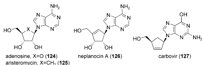
Figure 9. Representative carbocyclic nucleosides.
