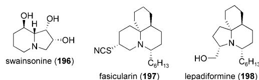
Figure 13. Representative indolizidine and pyrrolizidine alkaloids.
