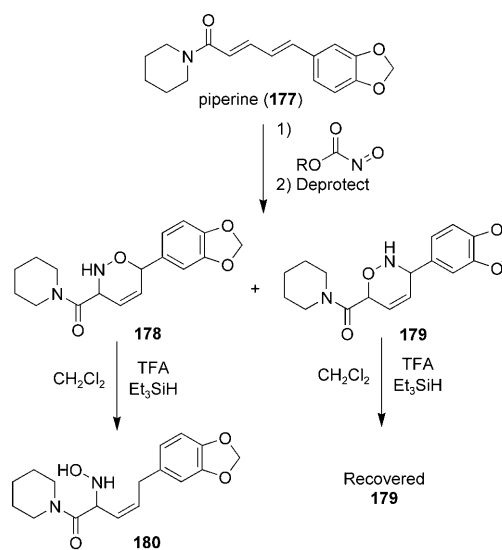
Scheme 32. A nitroso-Diels–Alder reaction with piperine ( 177 ). TFA = trifluoroacetic acid.
