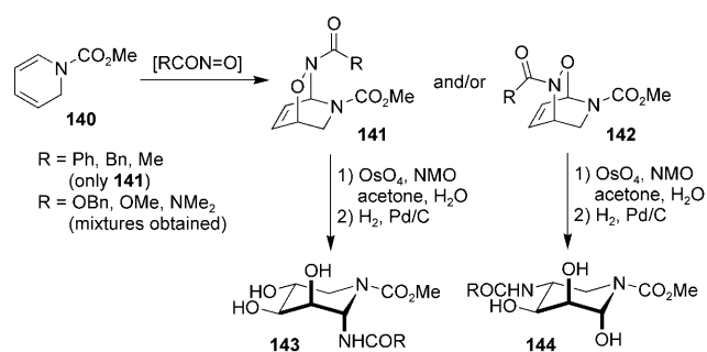
Scheme 27. Route to aza sugars from 1,2-dihydropyridines.
