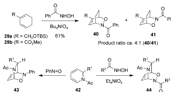
Scheme 7. Examples of regioselectivity in nitrosocarbonyl HDA reactions. TBS = tert -butyldimethylsilyl.
