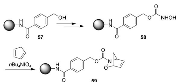
Scheme 10. Nitrosocarbonyl HDA reaction on a solid phase.
