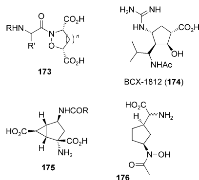
Figure 12. Representative amino acid derivatives and related structures.
