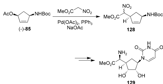
Scheme 24. Synthesis of the carbocyclic uracil polyoxin C.
