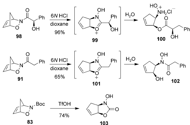
Scheme 18. Brønsted acid mediated cleavage of a C–O bond. TfOH = trifluoromethanesulfonic acid.
