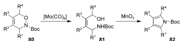
Scheme 14. Pyrrole synthesis by reductive cleavage of a N–O bond. Boc = tert -butoxycarbonyl.
