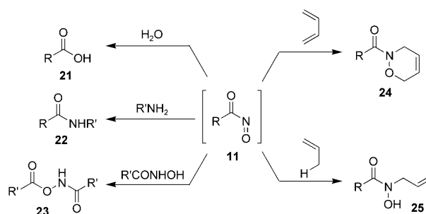
Scheme 3. Reactions of nitrosocarbonyl compounds.
