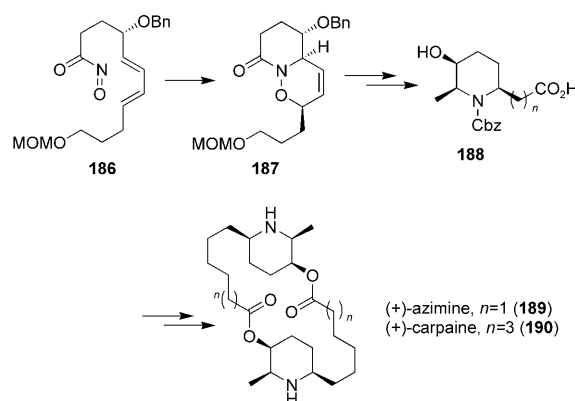
Scheme 35. Synthesis of (+)-azimine and (+)-carpine.
