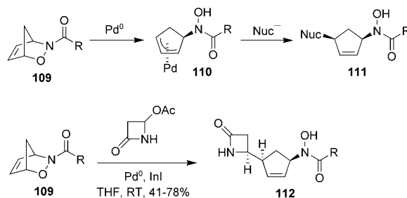
Scheme 21. Pd/In-mediated cleavage of a C–O bond.
