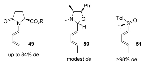
Figure 8. Examples of chiral acyclic dienes.
