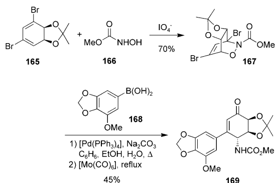
Scheme 30. Synthetic route to narciclasine.
