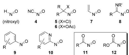
Figure 1. Examples of C-nitroso compounds.
