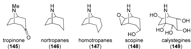
Figure 10. Structures of the tropane alkaloid family.
