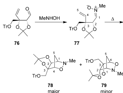
Scheme 13. [3+2] Cycloaddition for the synthesis of 3,6-dihydro-1,2-oxazines. Tr = triphenylmethyl.
